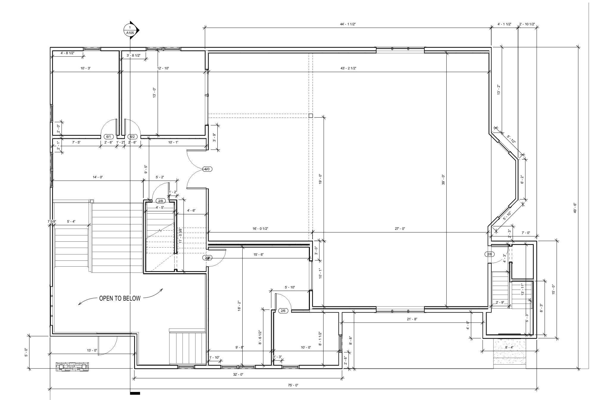
① MAIN FLOOR 1/4" = 1'-0"
